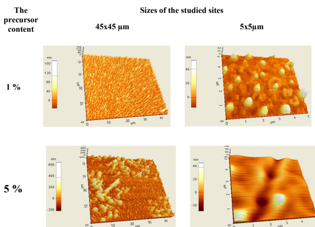
Fig. 2. AFM-images of the surfaces of tin dioxide films obtained from precursor complex number 2. The precursor content and the sizes of the studied sites are indicated.
