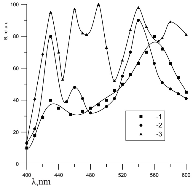
Fig. 2. Spectral distribution of the PL (1), electroluminescence (2) and LEIE (3) \text{Ta}_2\text{O}_5 films in contact with the electrolyte.
