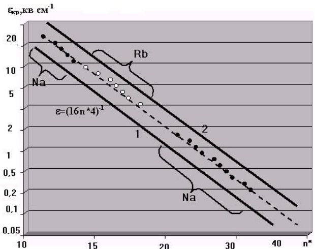
Fig.1. Critical electric field strength \epsilon_{sp} in dependence upon effective quantum number n^* for atoms of Na, Rb: dots – experiment (see [1]); solid line 1 – theoretical estimate on the basis of classical model; solid line 2 – calculation within the H-like approximation; dotted line – our data (eq.(1))
